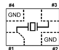
Top view connections #2 & #4: connected to metal lid
