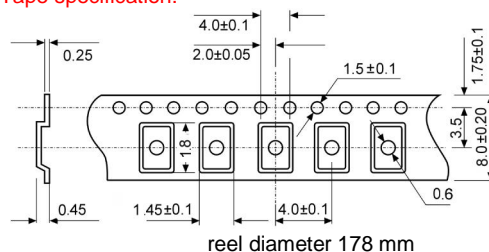
reel diameter 178 mm
